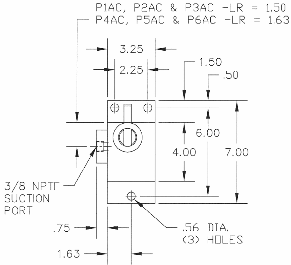
TOP VIEW ROATATE 90° CCW
