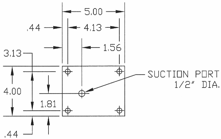
HOLE PATTERN FOR RESERVOIR AND GASKET—VIEW A-A
